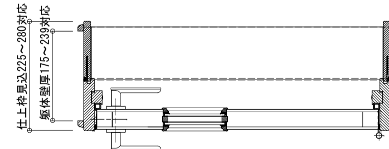
DFGN0820AD/L + DFT0828AD/L(付枠)
