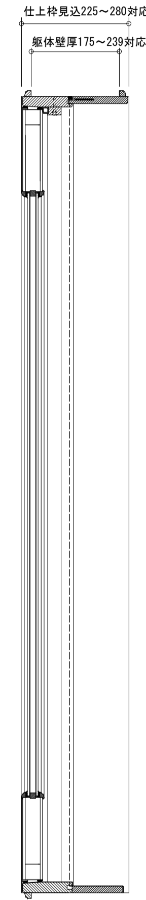
DFGN0820AD/L + DFT0828AD/L(付枠)
