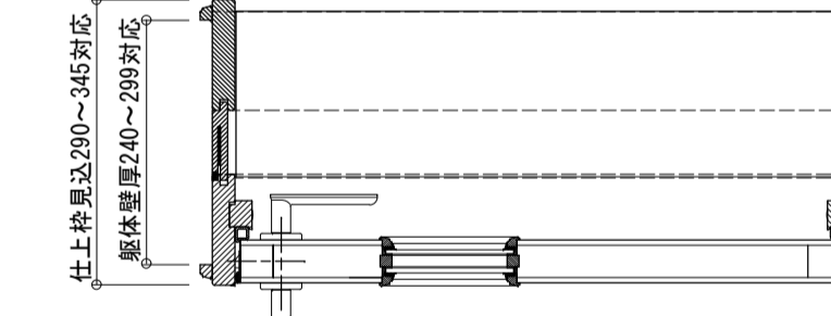
DFGN0820AD/L + DFT0834AD/L(付枠)
