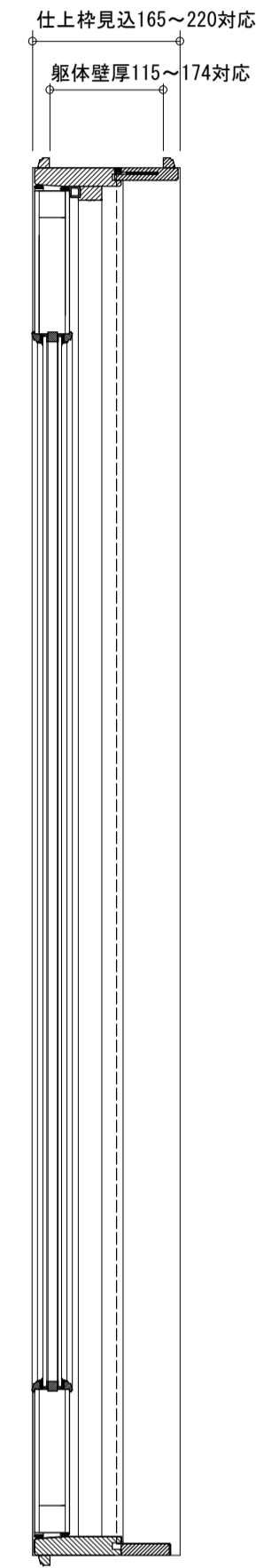
DFGN0820AD/L + DFT0822AD/L(付枠)
