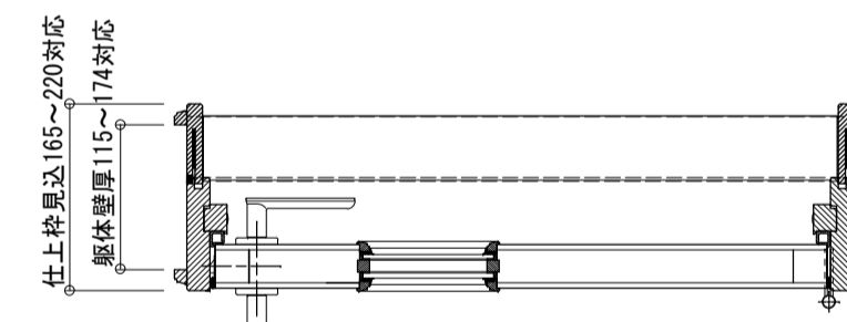
DFGN0820AD/L + DFT0822AD/L(付枠)
