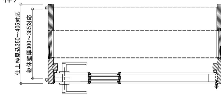
DFGN0920AD/L + DFT0940AD/L (付枠)
