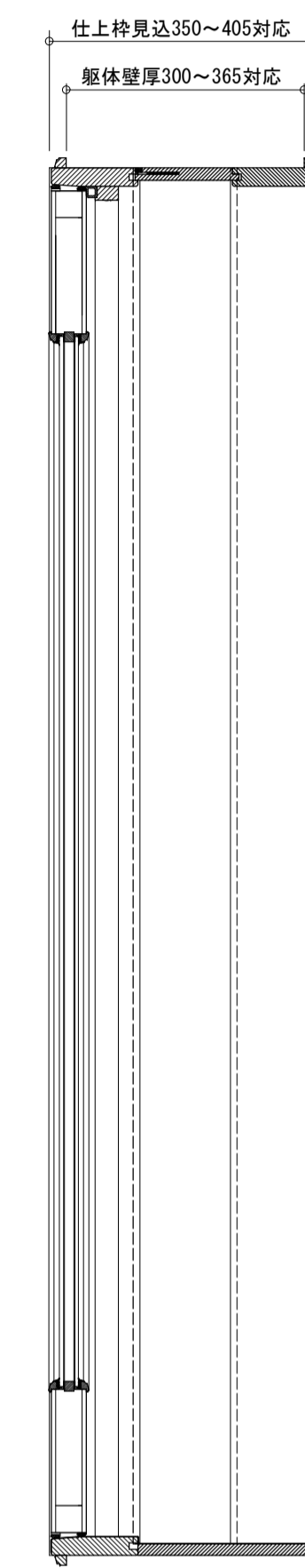
DFGN0920AD/L + DFT0940AD/L (付枠)
