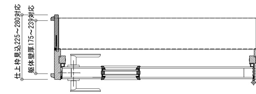
DFGN0920AD/L + DFT0928AD/L (付枠)
