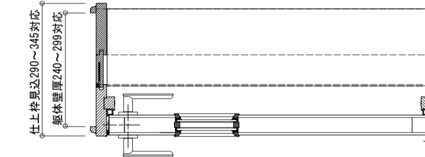
DFGN0920AD/L + DFT0934AD/L (付枠)
