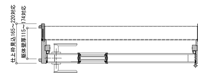
DFGN0920AD/L + DFT0922AD/L (付枠)
