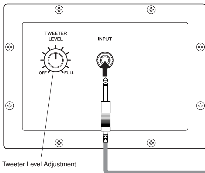
[Speaker System Rear Panel]
