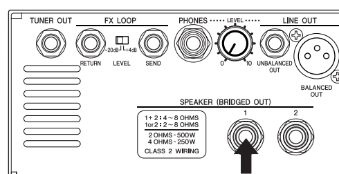
Speaker Output Jack on the Head Amplifier/Power Amplifier.
